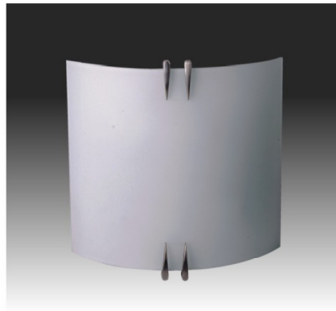
MODEL NO: DWS3138 SIZE: 10"L x 11-1/4"W x 3-3/4"E LAMP/WATTAGE: 2 x 18W PLC
