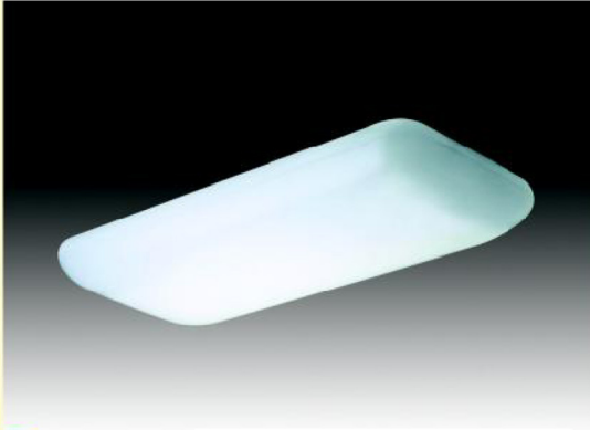
MODEL NO: CWA-24-2L-T8/17W-120V SIZE: 26-1/2"L x 11-5/8"W x 4-1/2"H LAMP/WATTAGE: 2 x T8/17W, 2 x T12/20W
