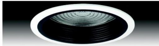
MODEL NO: RT-6-CF-BB-FL-2-13W-HL DESCRIPTION: BLACK BAFFLE/ FRESNEL LENS SIZE: 7-1/8" DIA LAMP/WATTAGE: 2 x 13W QUAD LAMP
